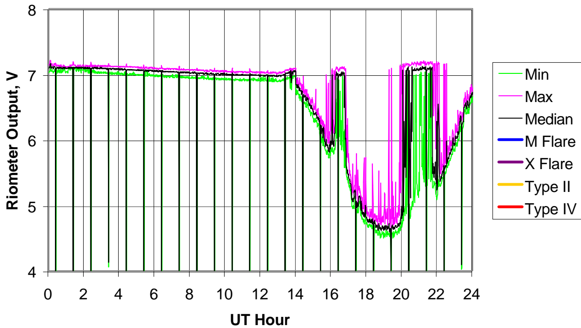
BLO Riometer, 2005 Day 241 (29 Aug 2005)
