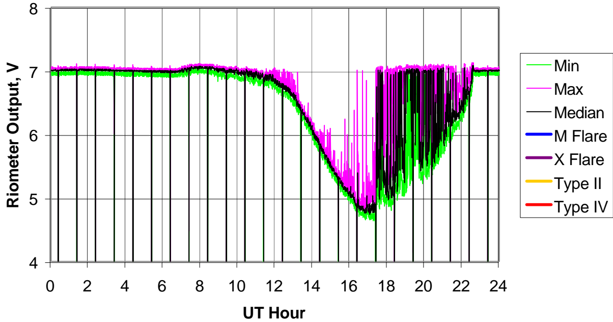
BLO Riometer, 2005 Day 267 (24 Sep 2005)
