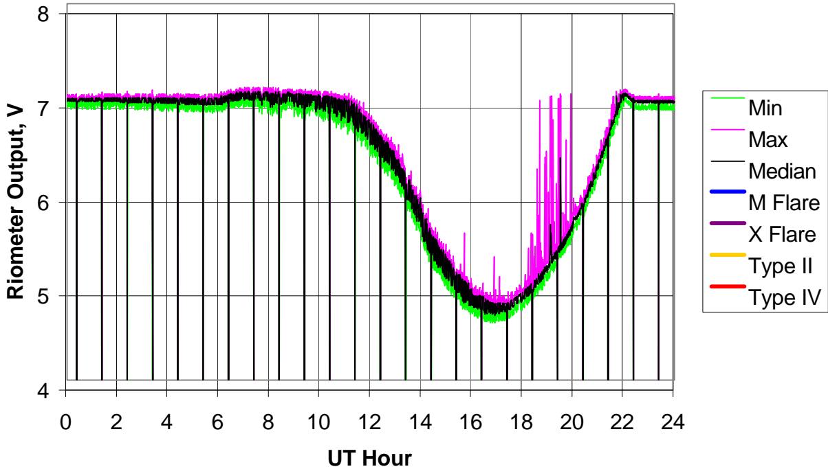
BLO Riometer, 2005 Day 281 (08 Oct 2005)
