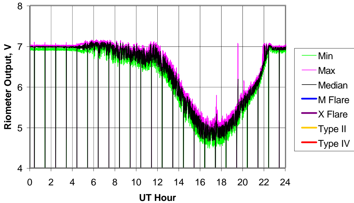
BLO Riometer, 2005 Day 276 (03 Oct 2005)
