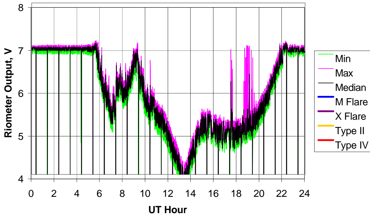
BLO Riometer, 2005 Day 277 (04 Oct 2005)
