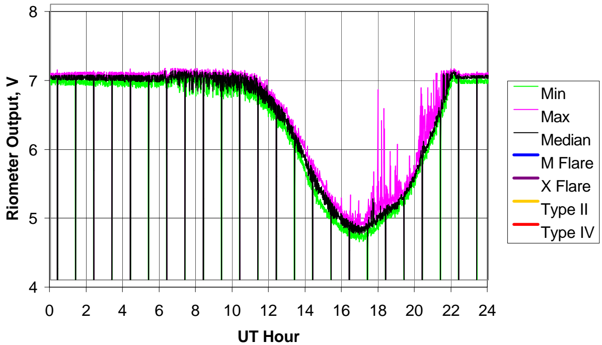
BLO Riometer, 2005 Day 278 (06 Oct 2005)
