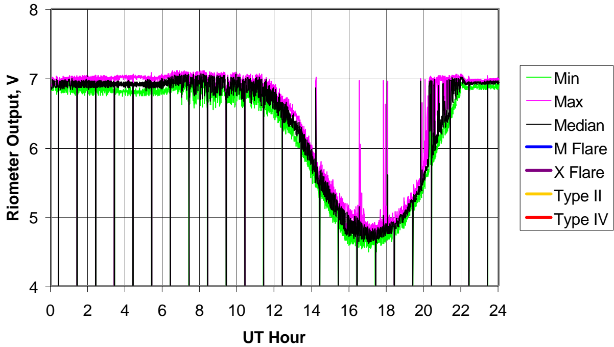
BLO Riometer, 2005 Day 278 (05 Oct 2005)
