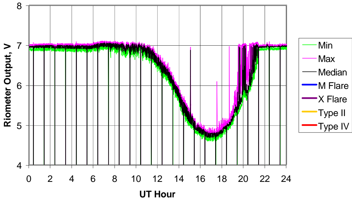
BLO Riometer, 2005 Day 280 (07 Oct 2005)
