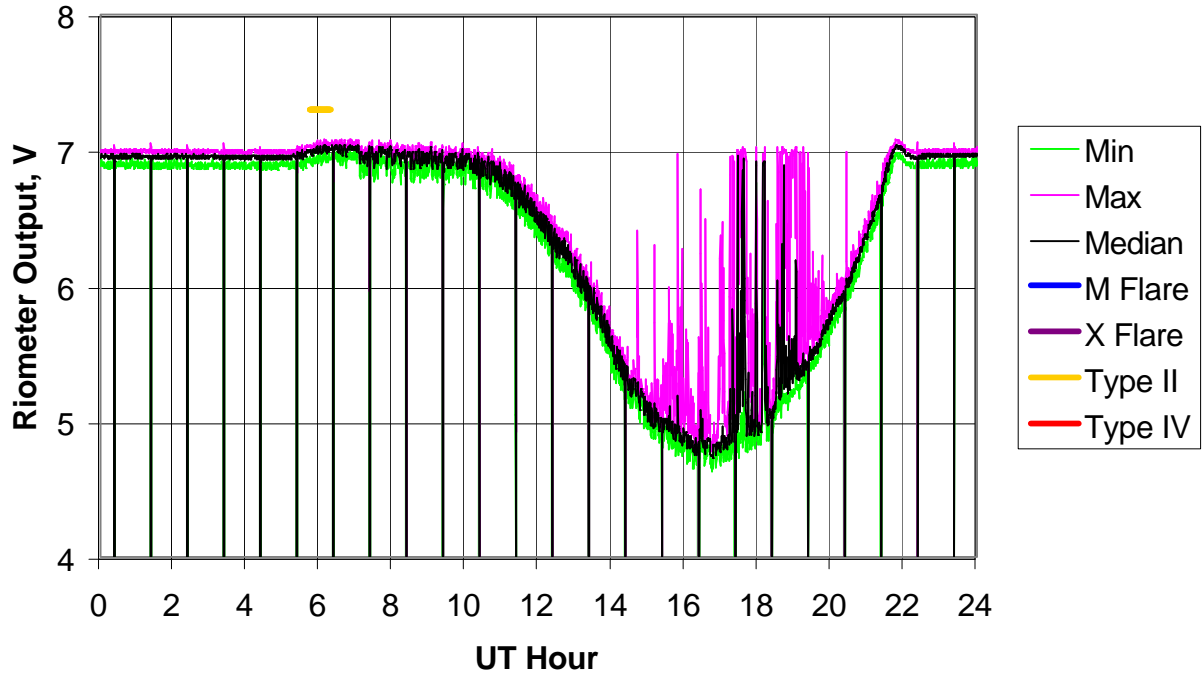
BLO Riometer, 2005 Day 285 (12 Oct 2005)
