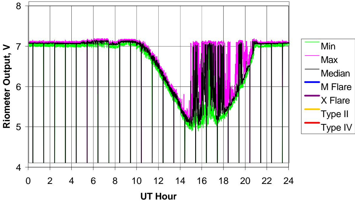
BLO Riometer, 2005 Day 295 (22 Oct 2005)
