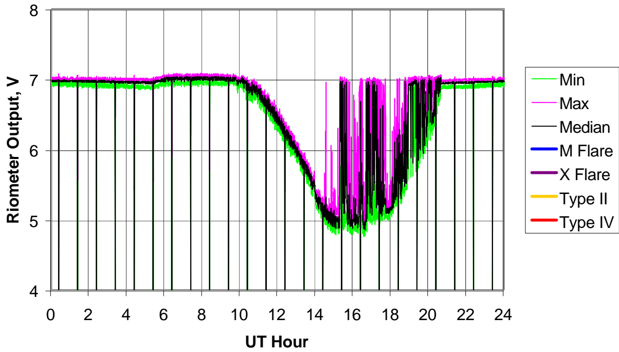
BLO Riometer, 2005 Day 294 (21 Oct 2005)
