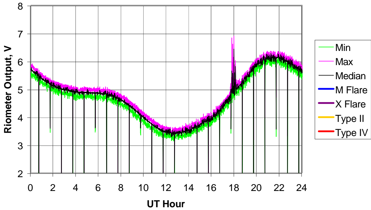
BLO Riometer, 2005 Day 343 (09 Dec 2005)
