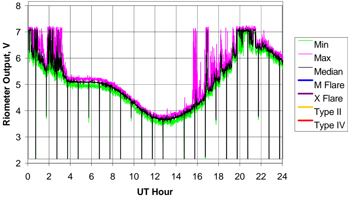
BLO Riometer, 2005 Day 340 (06 Dec 2005)
