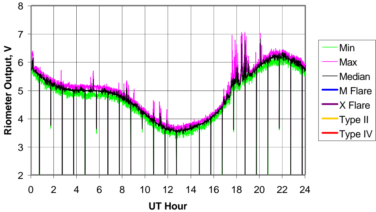
BLO Riometer, 2005 Day 341 (07 Dec 2005)
