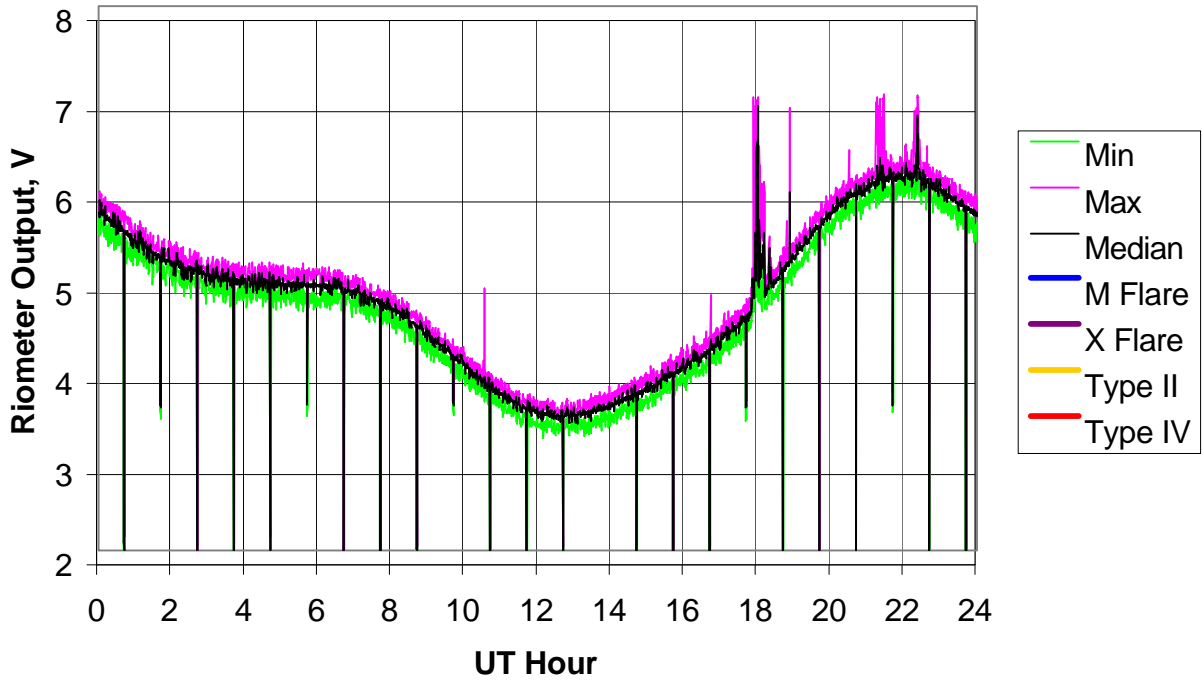
BLO Riometer, 2005 Day 342 (08 Dec 2005)
