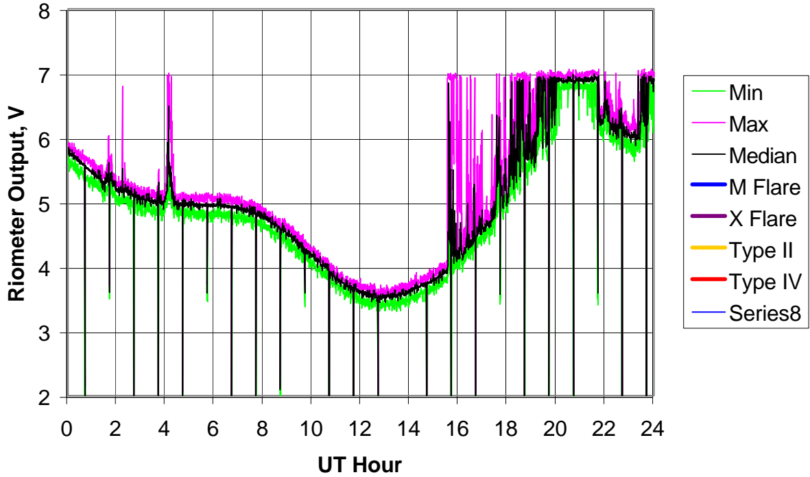
BLO Riometer, 2005 Day 339 (05 Dec 2005)
