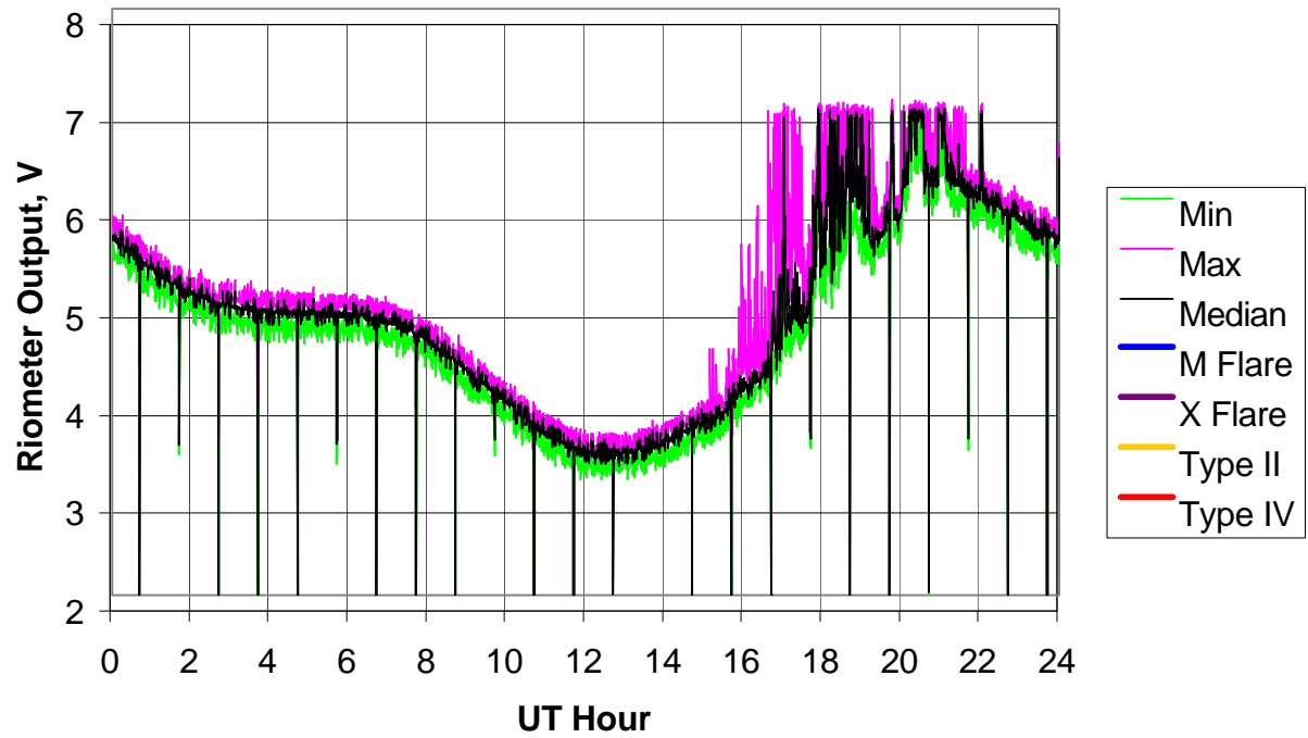
BLO Riometer, 2005 Day 344 (10 Dec 2005)
