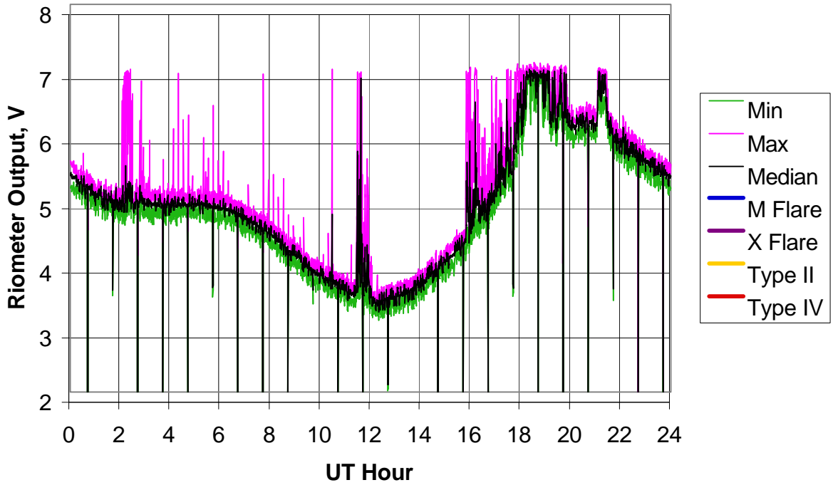
BLO Riometer, 2005 Day 356 (22 Dec 2005)
