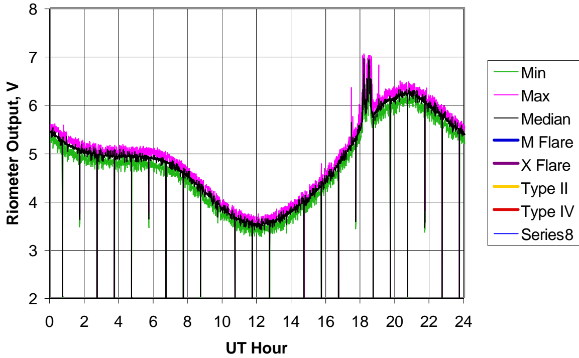
BLO Riometer, 2005 Day 353 (19 Dec 2005)
