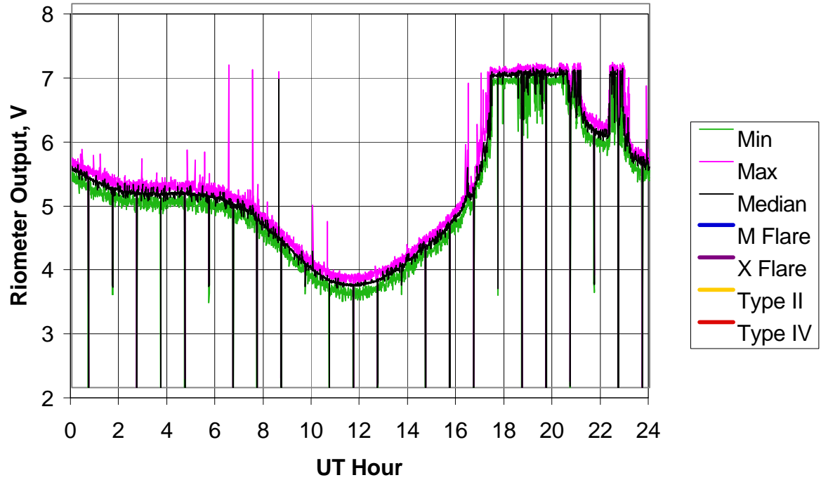
BLO Riometer, 2005 Day 358 (24 Dec 2005)
