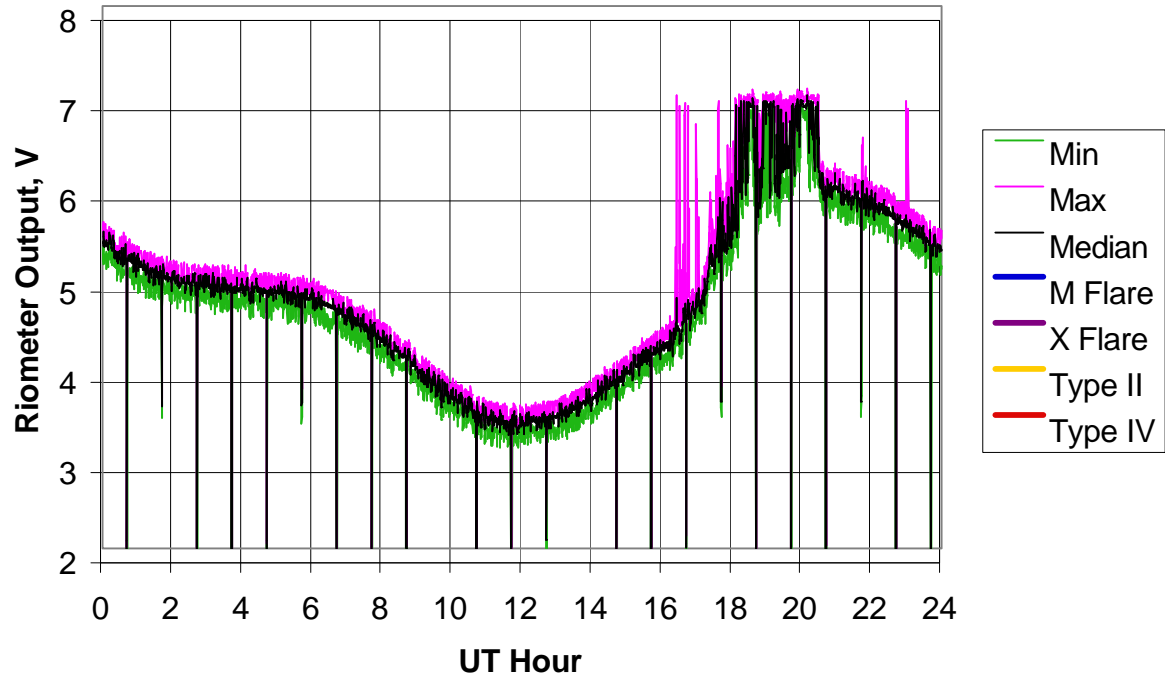
BLO Riometer, 2005 Day 354 (20 Dec 2005)
