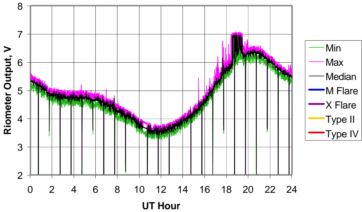
BLO Riometer, 2005 Day 357 (23 Dec 2005)
