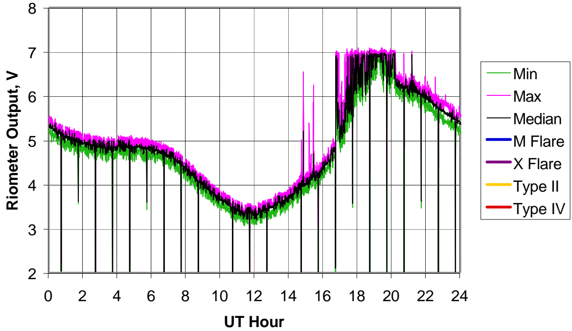
BLO Riometer, 2005 Day 355 (21 Dec 2005)
