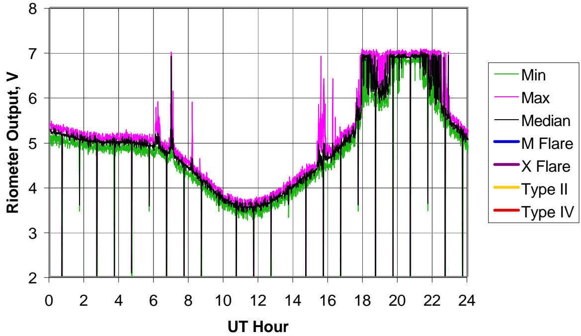
BLO Riometer, 2005 Day 362 (28 Dec 2005)
