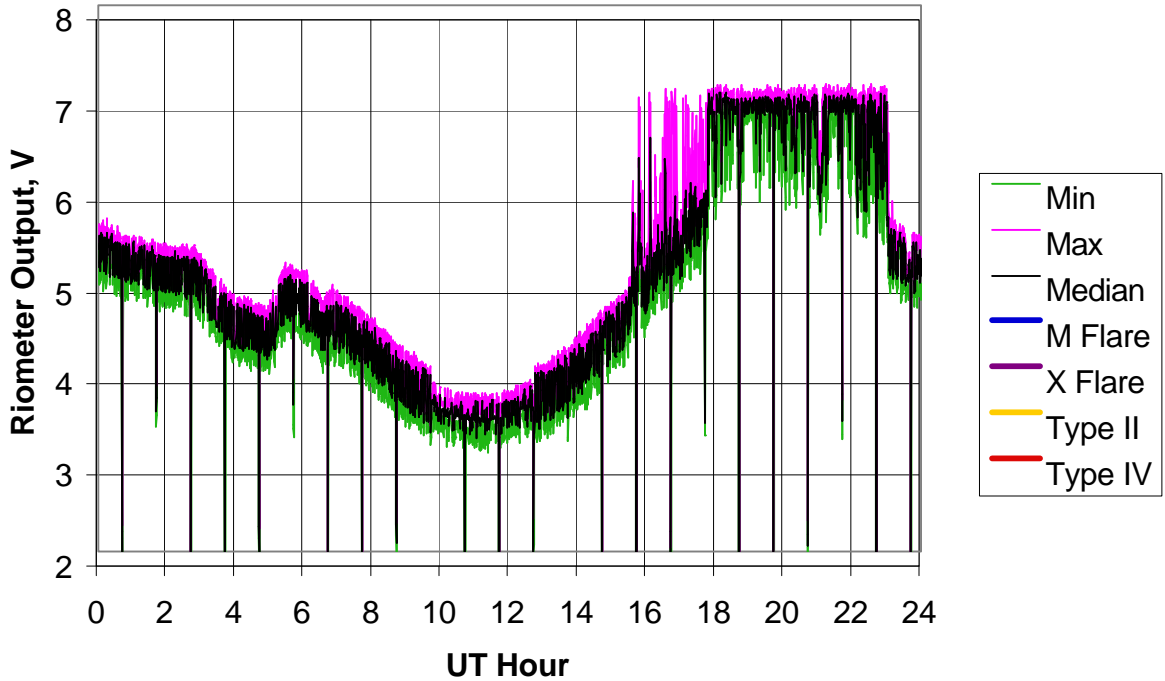
BLO Riometer, 2005 Day 365 (31 Dec 2005)
