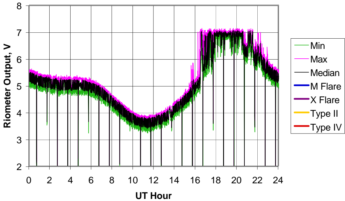
BLO Riometer, 2005 Day 364 (30 Dec 2005)
