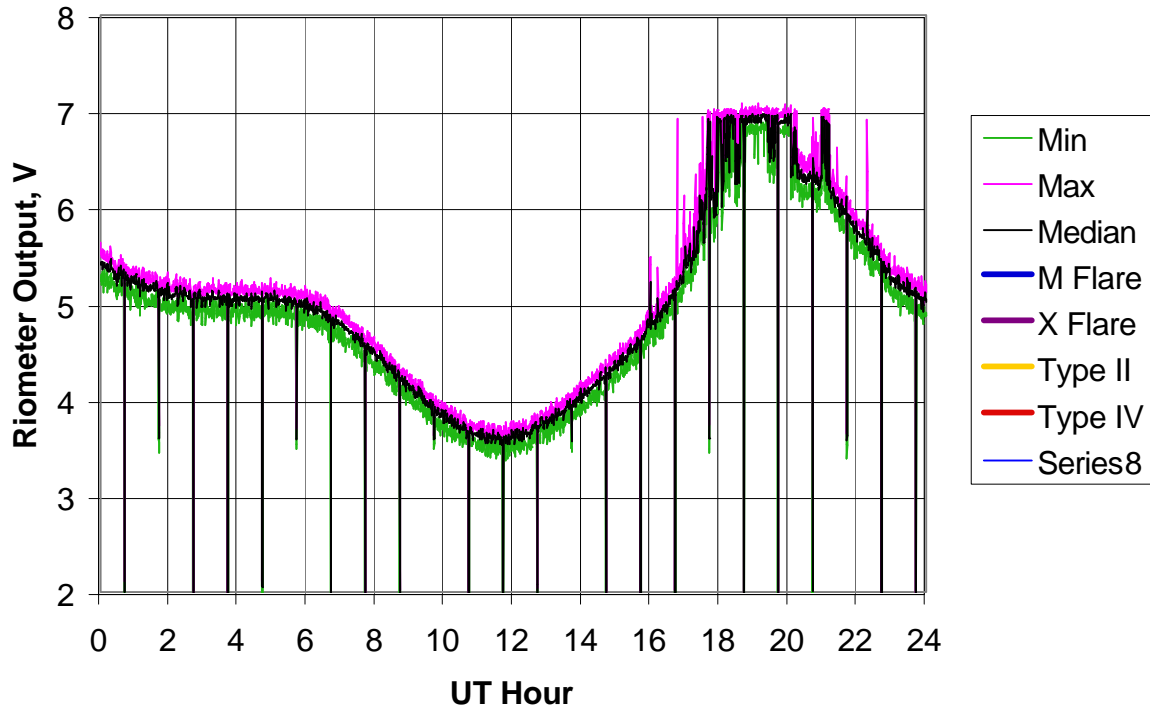
BLO Riometer, 2005 Day 360 (26 Dec 2005)
