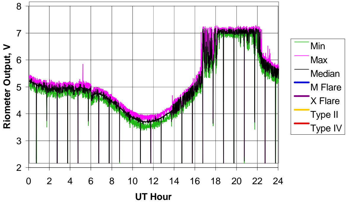
BLO Riometer, 2005 Day 363 (29 Dec 2005)
