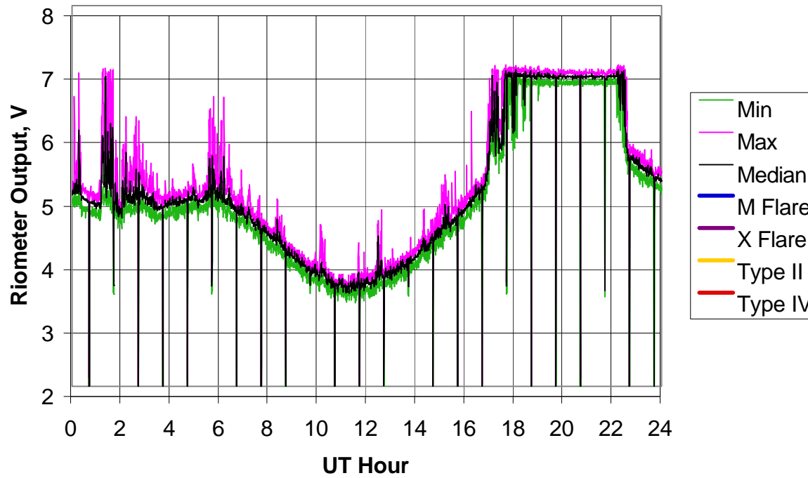
BLO Riometer, 2005 Day 361 (27 Dec 2005)
