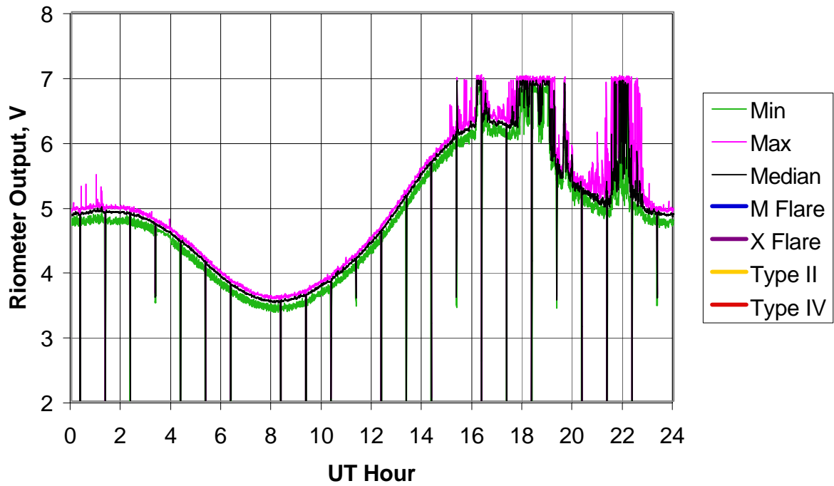
BLO Riometer, 2006 Day 048 (17 Feb 2006)
