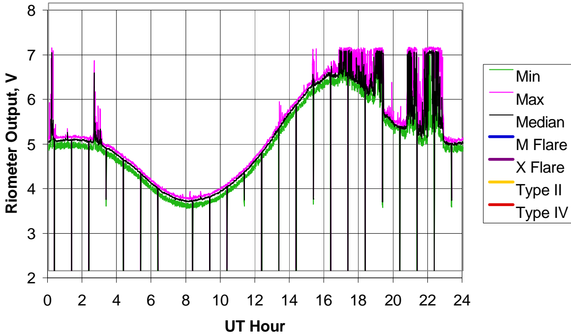
BLO Riometer, 2006 Day 047 (16 Feb 2006)
