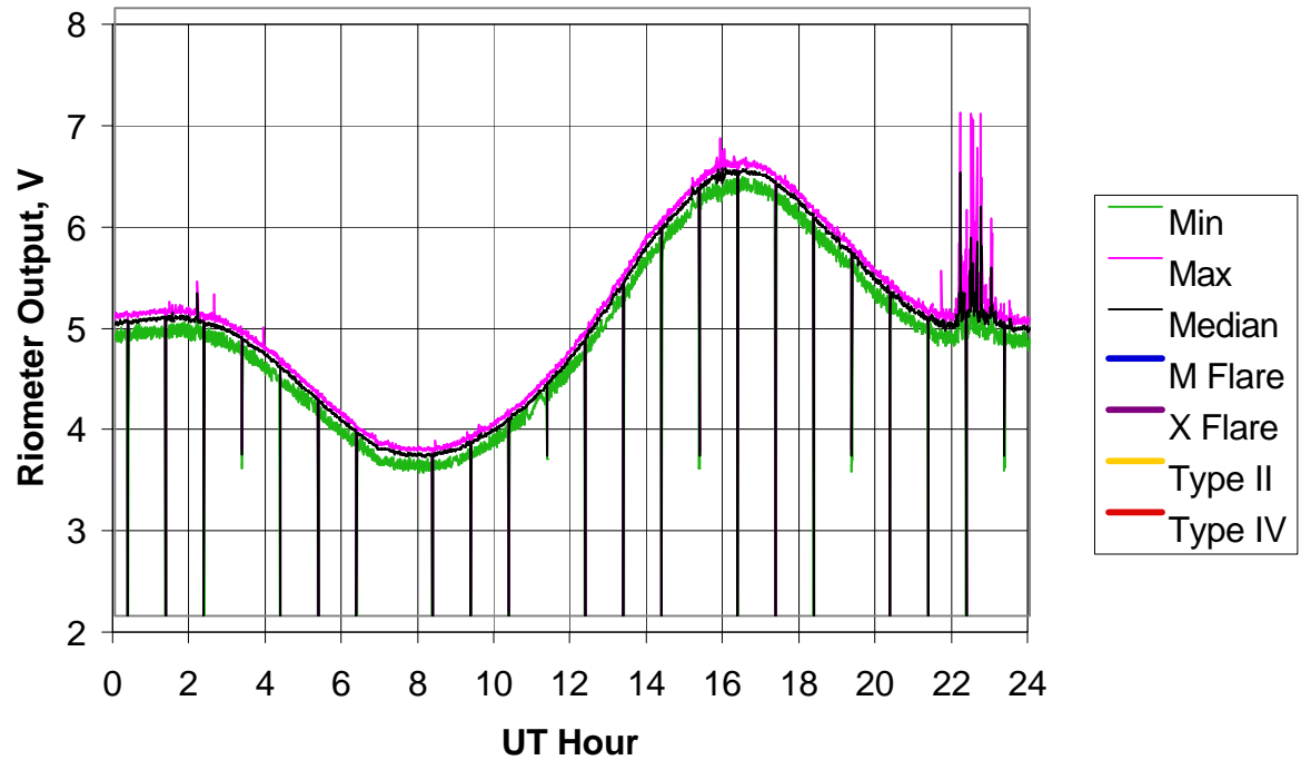
BLO Riometer, 2006 Day 049 (18 Feb 2006)
