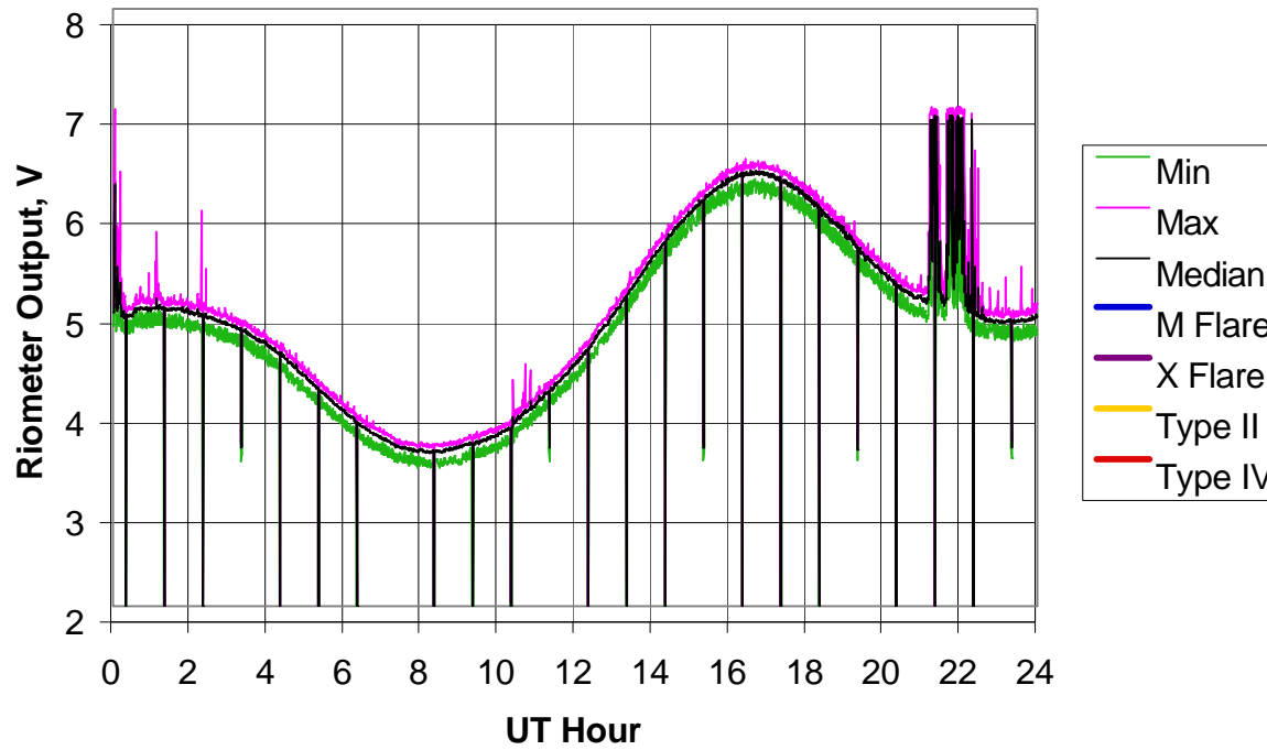
BLO Riometer, 2006 Day 045 (14 Feb 2006)
