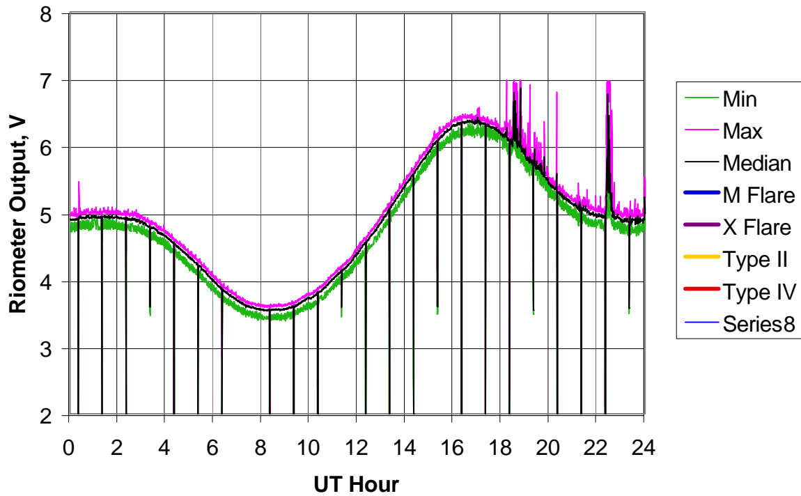
BLO Riometer, 2006 Day 044 (13 Feb 2006)
