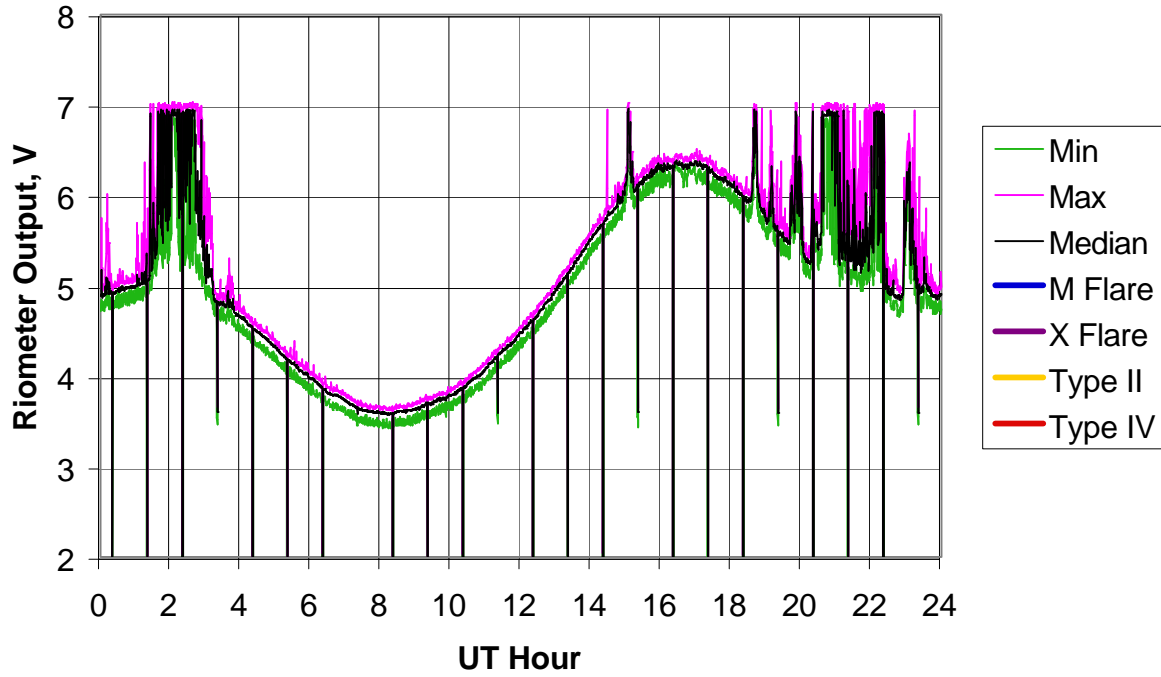
BLO Riometer, 2006 Day 046 (15 Feb 2006)
